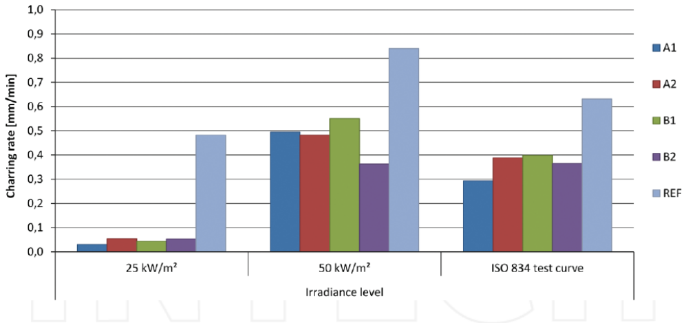
Figure 2. Charring rate of intumescent coated and uncoated wood exposed to different test conditions [29].
