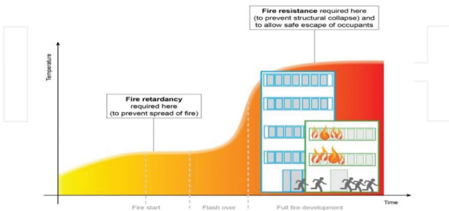
Figure 1. Phases of fire development in an enclosure.
